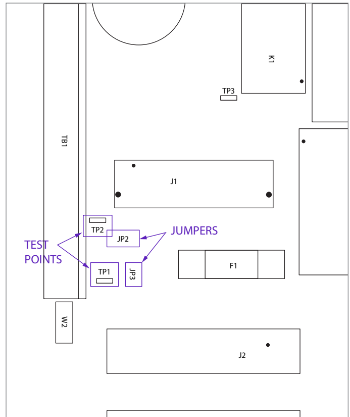
Figure 5 - FRBii Jumpers and Test Points
