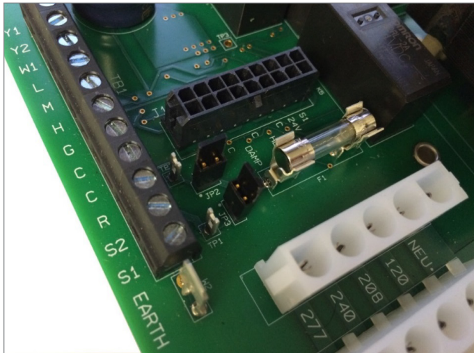
Figure 4 - Fan Relay Board (FRBii)
