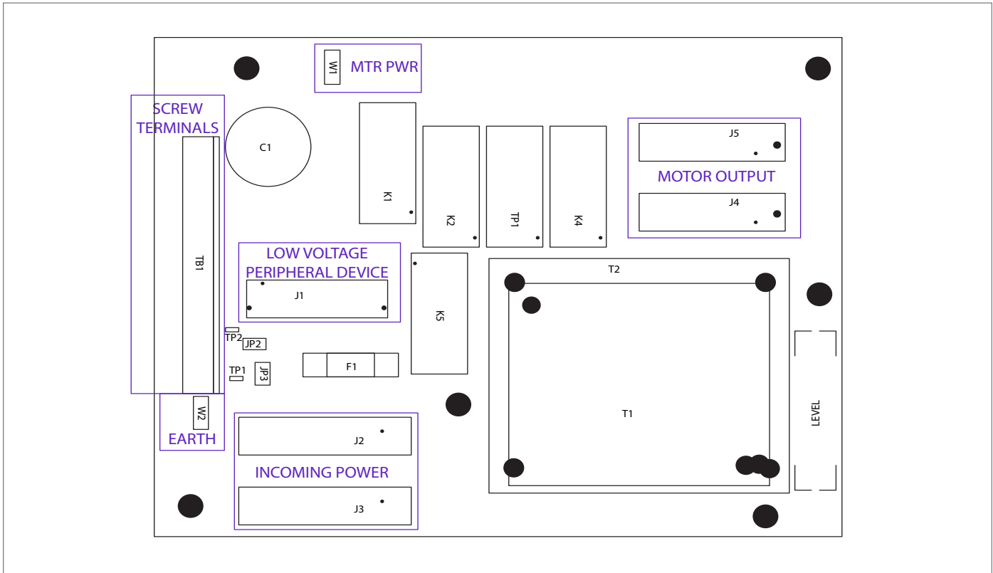
Figure 3 – Connector Layout
