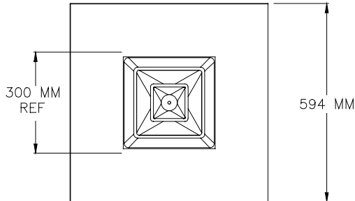
FACE VIEW FRAME 12 600 x 600
