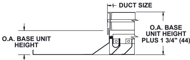
OBD1240 DETAIL TYPICAL OF ALL FRAME STYLES FR 23 SHOWN
