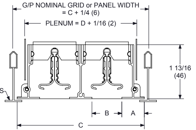
SECTION A-A WITH BLADES
