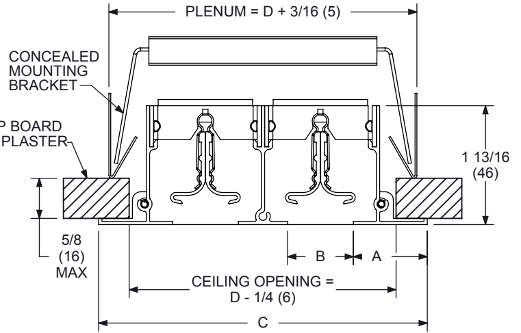
SECTION A-A WITH BLADES
