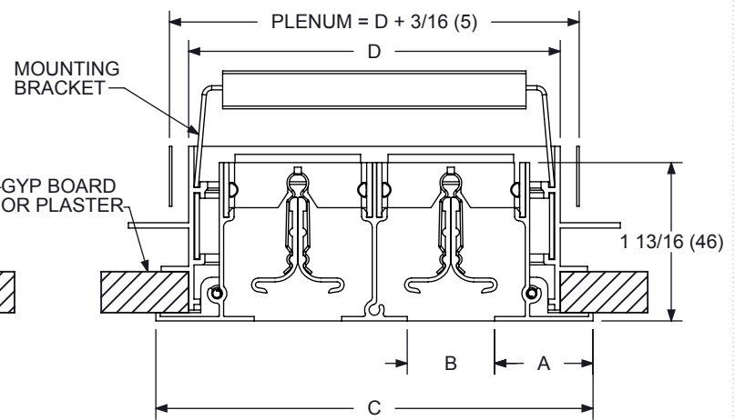
SECTION A-A WITH BLADES
