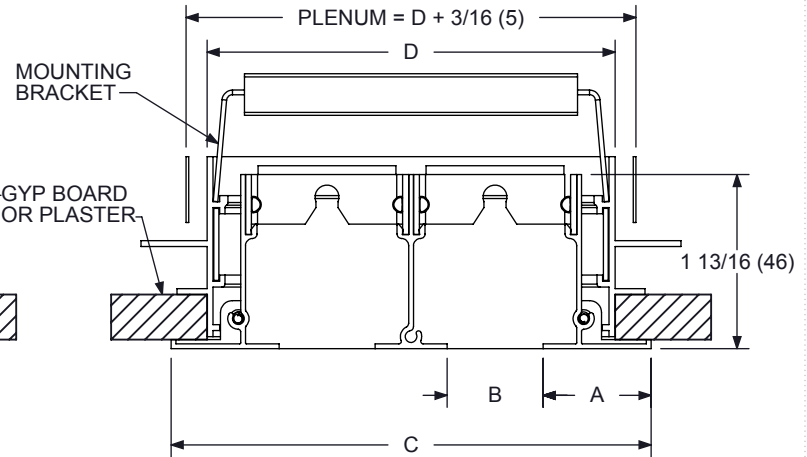
SECTION W-W NO BLADES
