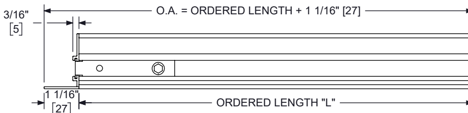
END CAP FACE VIEW
