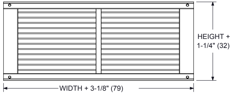
5DMGSUH FACE VIEW
