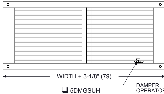
5DMGSUH FACE VIEW
