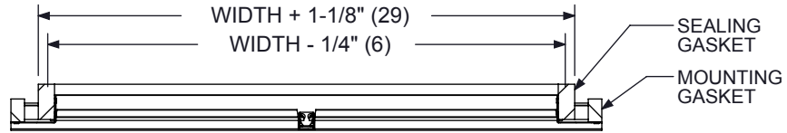
5DMGSUH TOP SECTION VIEW
