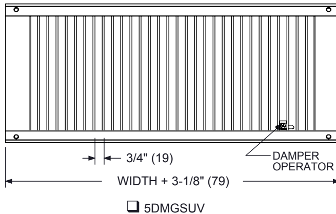
5DMGSUV FACE VIEW
