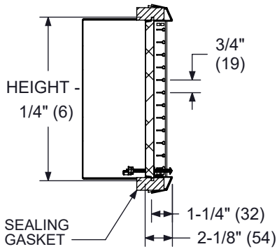
SIDE SECTION VIEW
