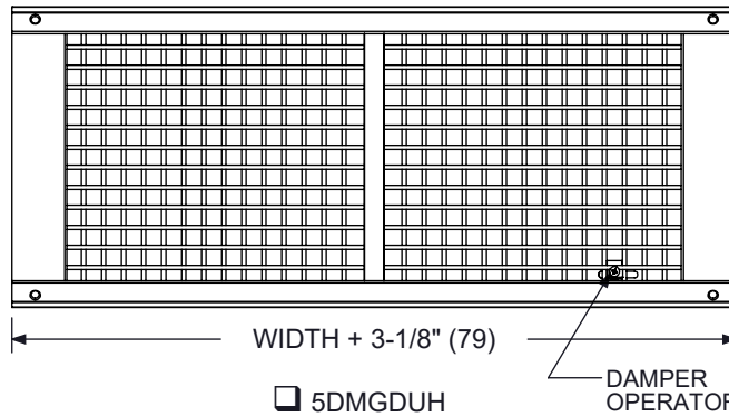
5DMGDUH FACE VIEW
