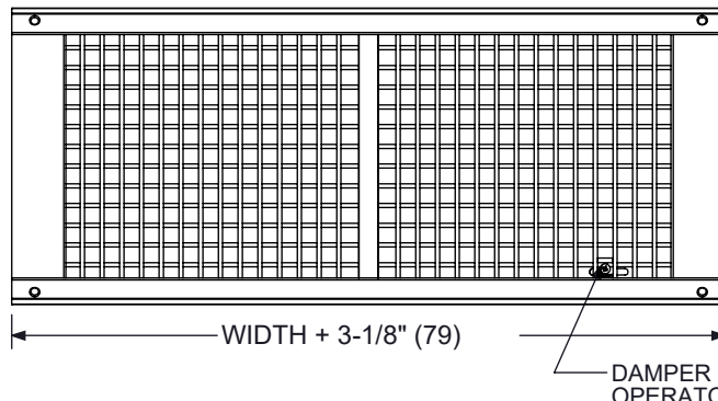
5DMGDUV FACE VIEW
