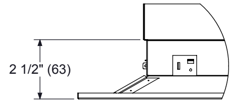
FACE TO NECK DIMENSION (SCREWS NOT SHOWN)
